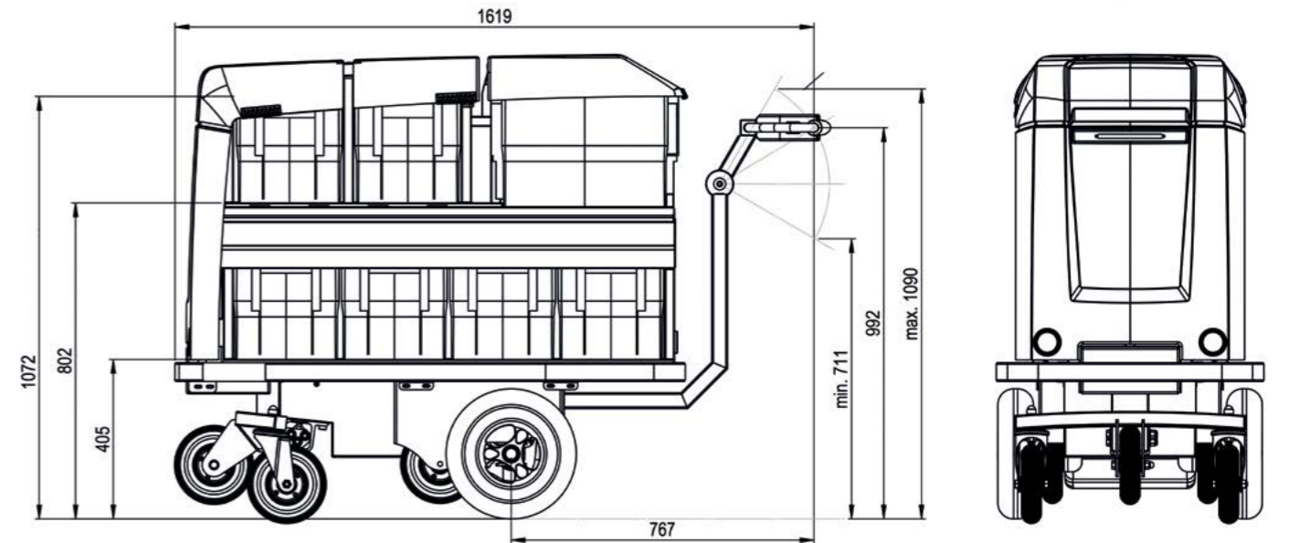
eTrolley 7+1
